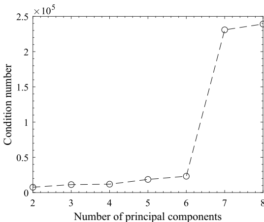
Fig. 17 Effect of the number of principal components on the condition number of the calibration matrix.
