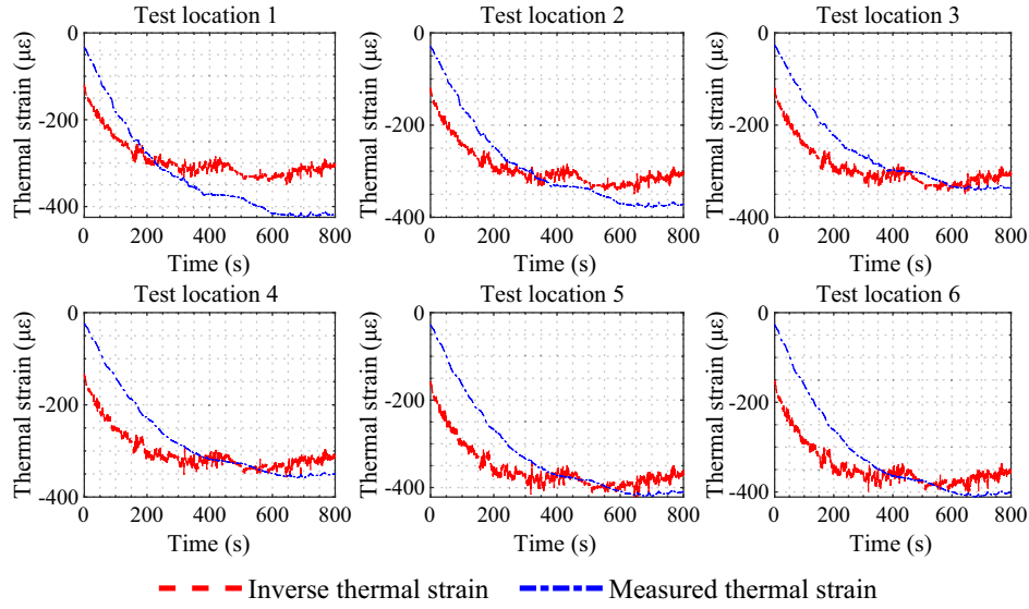
Fig. 11 Comparison of thermal strain at test locations.
