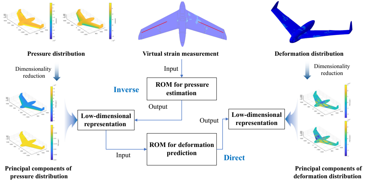
Fig. 2 Workflow for generating the improved inverse-direct load monitoring model using the simulation database (ROM, Reduced-order Model).
