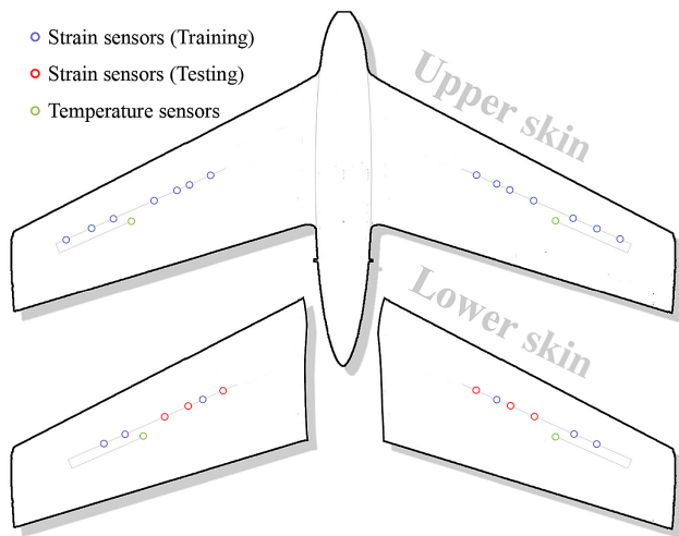
Fig. 6 Schematic layout of FBG sensors.
