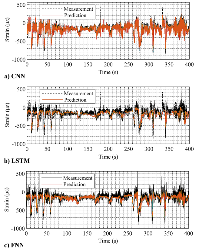
Fig. 13 Comparison of strain predictions for the proposed CNN-based model with the LSTM-based and FNN-based model at the first test sensor position.
