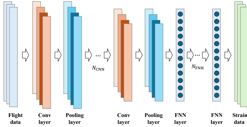
Fig. 3 CNN-based strain prediction neural networks.
