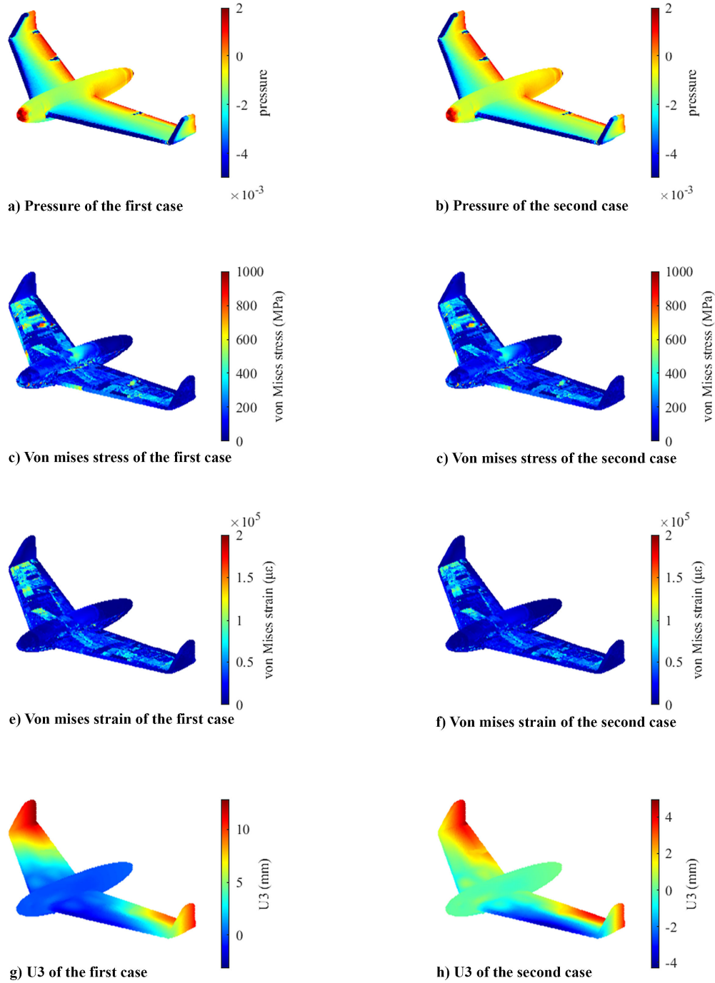
Fig. 15 Full-field deformation prediction with flight parameters as input at two different timestamps.
